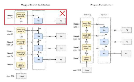
Figure 3.24. Removing stage 5 from the model.
