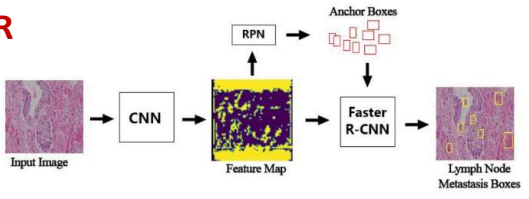
Figure 3.10. Faster R-CNN architecture
